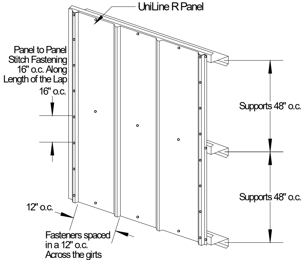
TYPICAL ASSEMBLY ISOMETRIC VIEW
